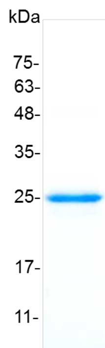
SDS-PAGE analysis of recombinant mouse IL-27 EBI3
